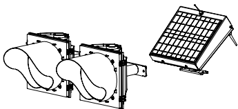
ISO VIEW
