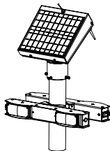
ISO VIEW
